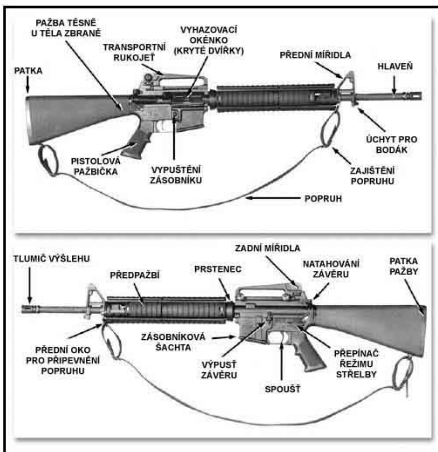
Obr. 3. Nomenclature, M16-series rifle (M16 - popis)
